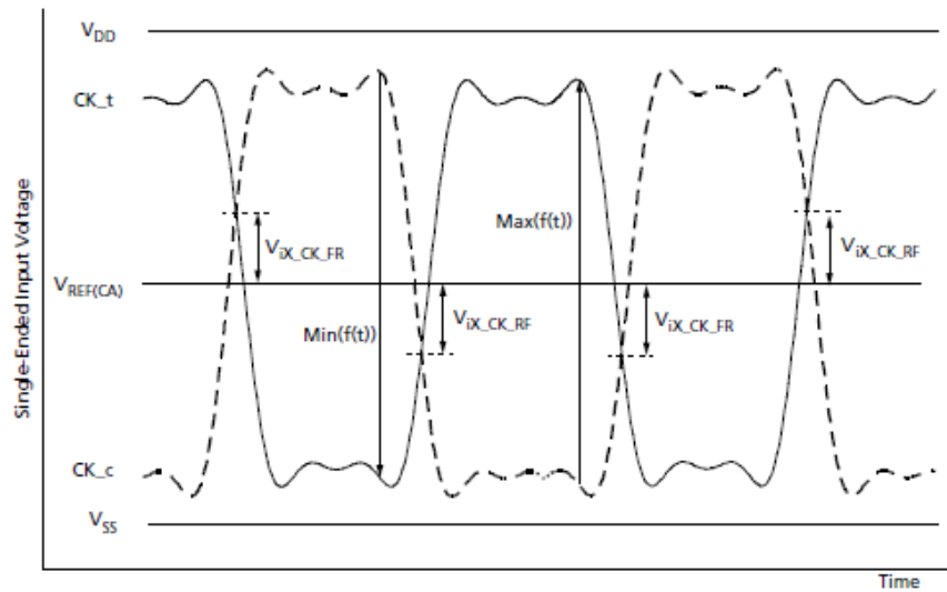
V_{ix} Definition (Clock)
