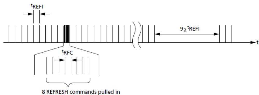
Pulling in REFRESH Commands (Example)
