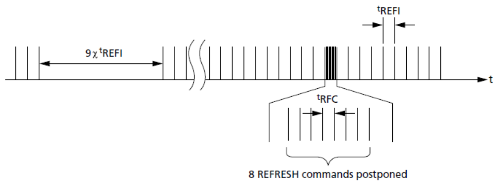
Postponing REFRESH Commands (Example)
